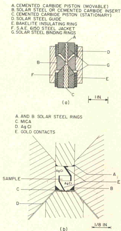
FIG. 3. (a) The piston-cylinder device which contains the high pressure at low temperatures. A thermocouple and a carbon resistor are located in holes drilled into part D. Four-lead resistance measurements are made between the top of piston A and the bottom of piston C. (b) A magnified view of the high-pressure sample chamber. All electrical contacts are pressure contacts. Electrical insulation is provided by mica C and AgCl D.
