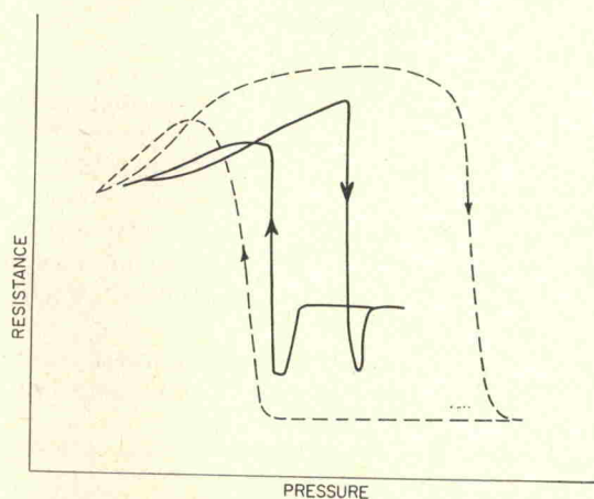
FIG. 4. Tracings taken from X-Y recorder plots showing electrical resistance as a function of applied pressure, both in relative units. The solid lines indicate a resistance versus pressure run at 249°K and the dashed line represents a run at 77°K. Note the difficulty of determining the beginning of the transition at 77°K. For this reason the pressure on the increasing stroke at half the discontinuity is used as the transition pressure.
